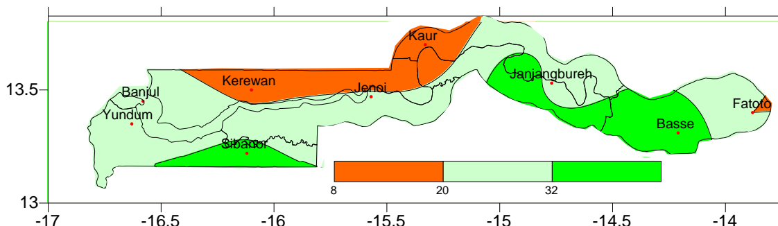
Figure 1a: Dekadal rainfall totals from 01st – 10 th October, 2018.
