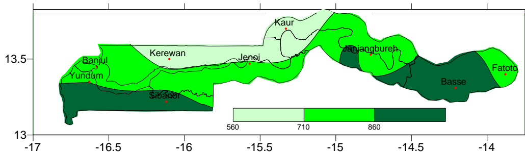
Figure 1b: Rainfall Seasonal totals from May 1 st 2018– October 10 th 2018.
