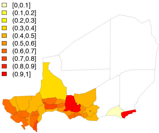
Sensitivity, Model 7
