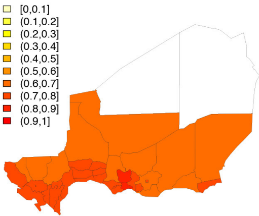
Specificity, Model 7
