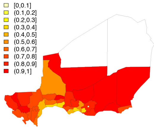
Specificity, Model 9
