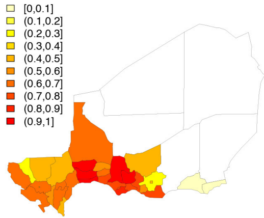
Sensitivity, Model 9
